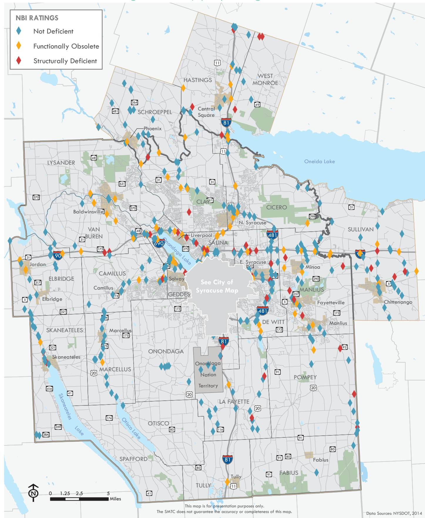
Exhibit 16: National Bridge Inventory (NBI) Ratings in the MPA
