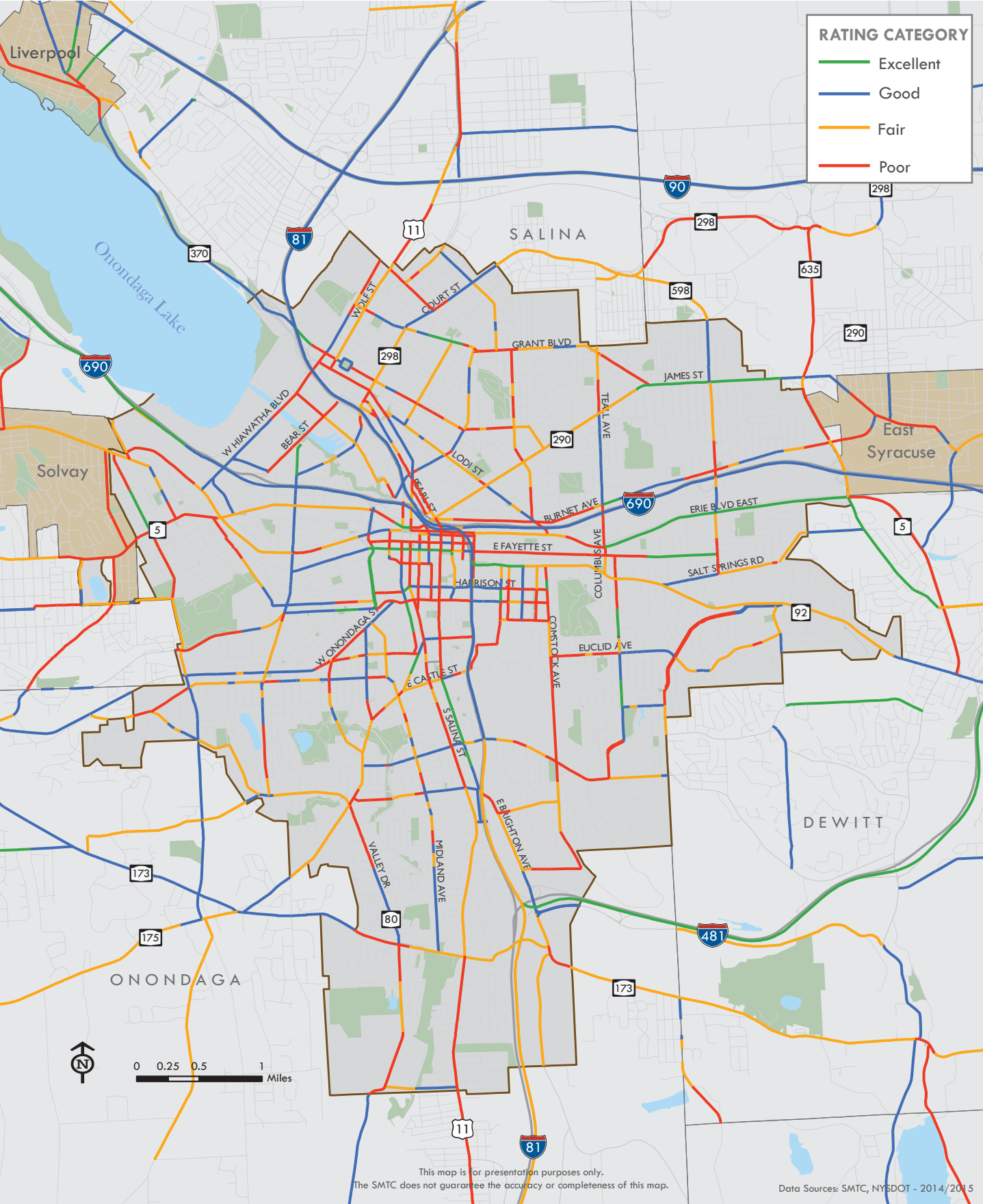
Exhibit 26: Pavement Ratings in the City of Syracuse
