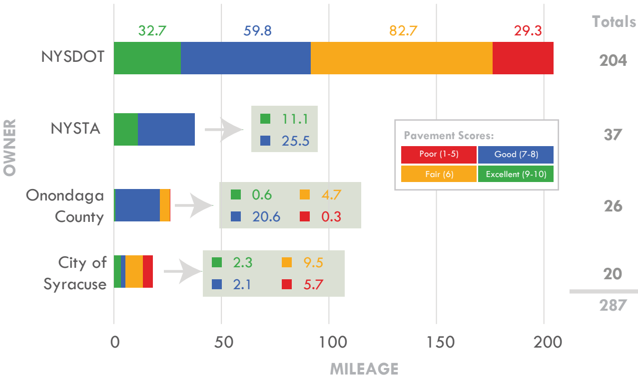
Exhibit 20: Pavement Ratings for Principal Arterials, by Mileage, Rating Category, and Owner
