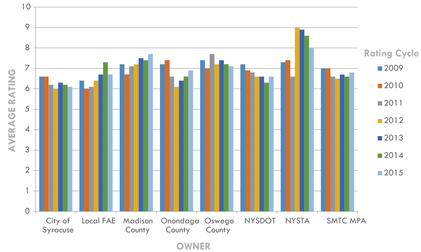
Exhibit 31: Trends of Average FAE Ratings in the MPA, by Owner
